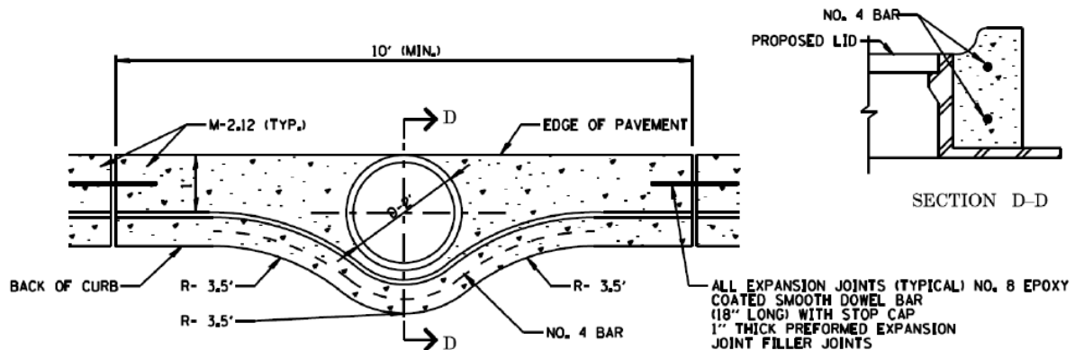
FIGURE 4-1 Detail of Curb and Gutter Inlet Structure
