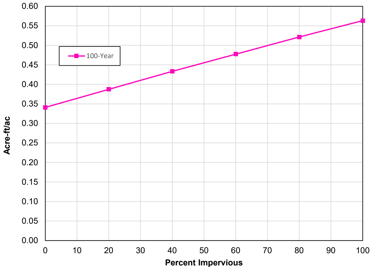
Figure 3.1 Detention Volume vs Percent Impervious Town of Dyer
