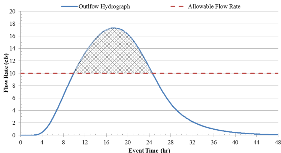
Figure 3.3 Required Storage Volume Determination Example
