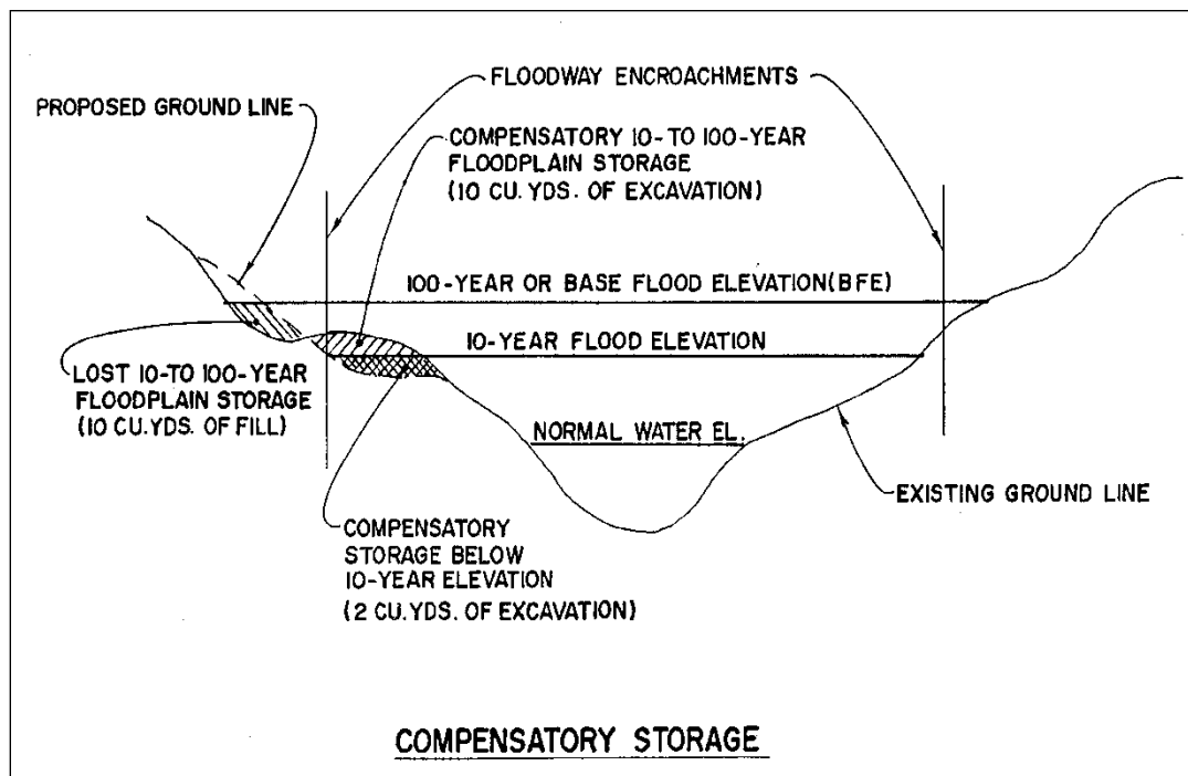
FIGURE 2.2 Compensatory Storage Example
