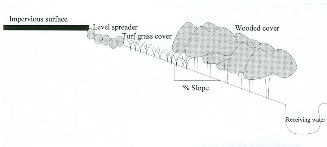
Figure PC-110A Typical Buffer Strip (SUSMP, 2002)
