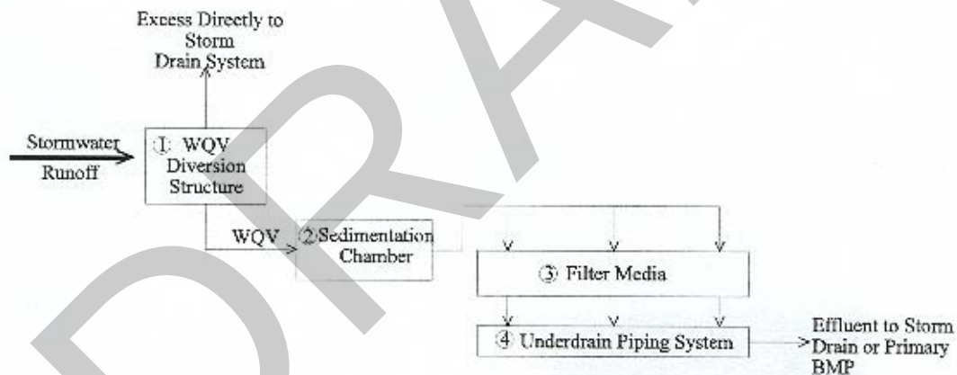
Figure PC-108A Typical Media Filtration Schematic (SUSMP, 2002)
